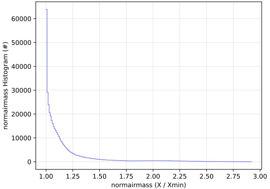
ddf_acor_sf30_lsf40_lsr20_v3.4_10yrs All sky z band: normairmass Histogram
