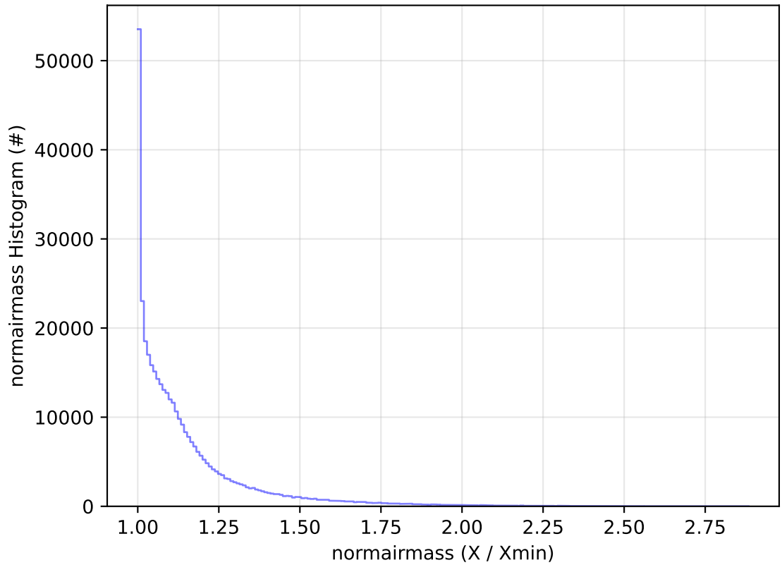
ddf_acor_sf30_lsf40_lsr20_v3.4_10yrs All sky y band: normairmass Histogram
