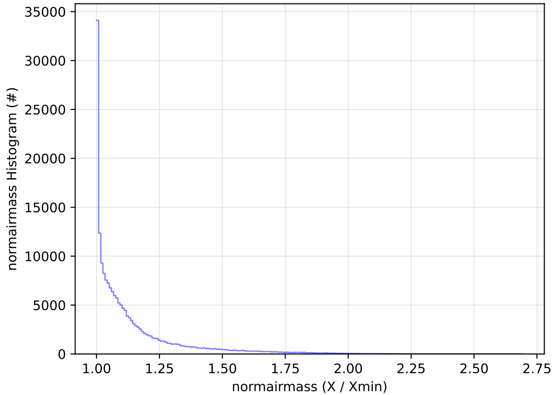
ddf_acor_sf30_lsf40_lsr20_v3.4_10yrs All sky g band: normairmass Histogram
