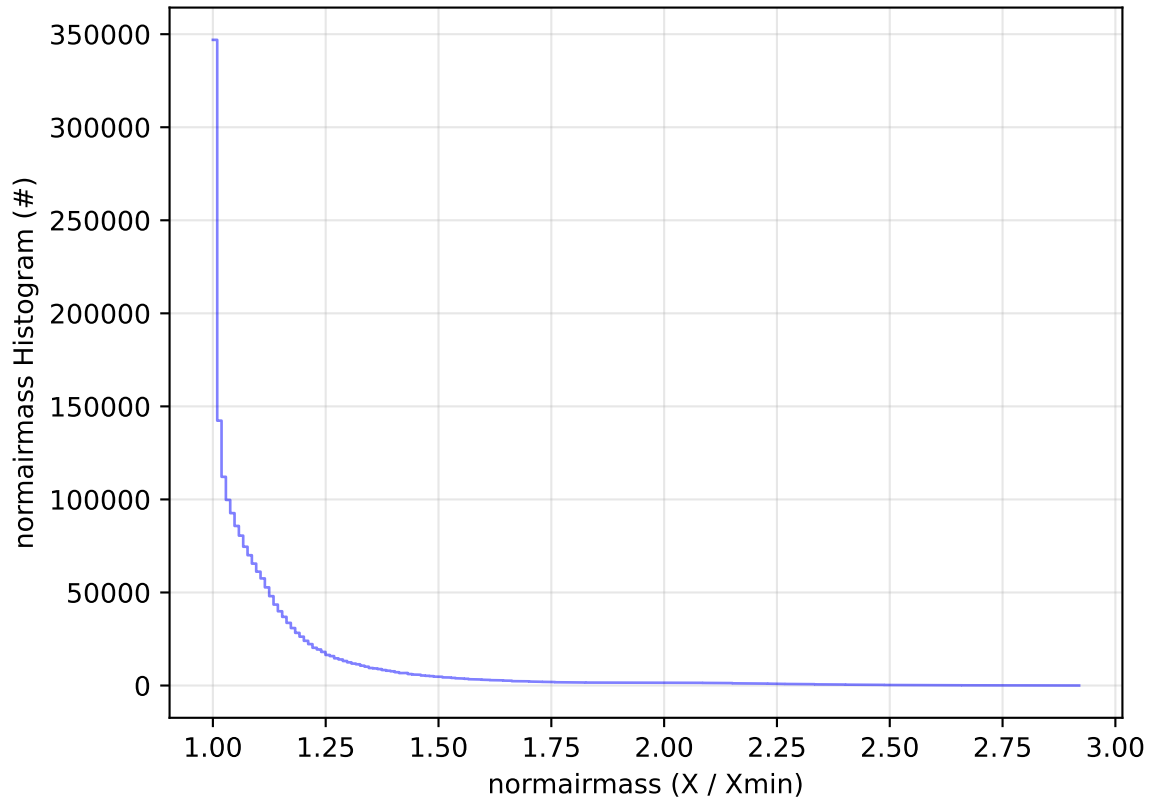
ddf_acor_sf30_lsf40_lsr20_v3.4_10yrs All sky all bands: normairmass Histogram
