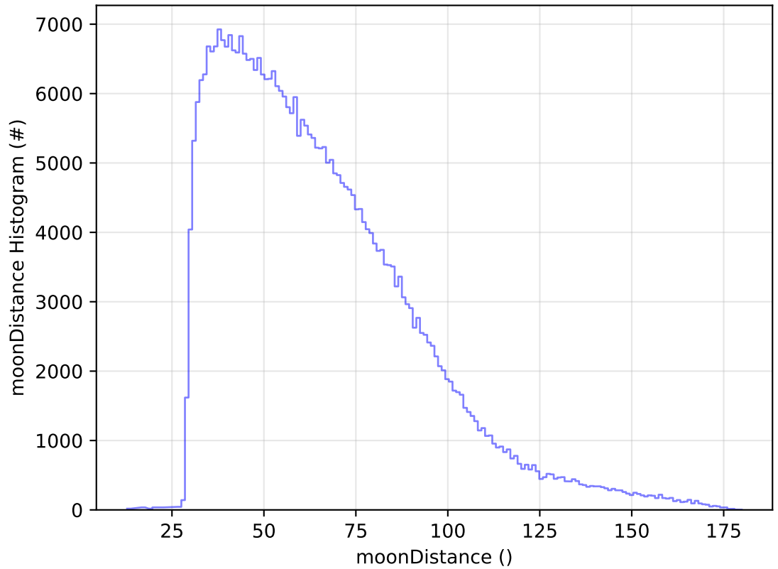
ddf_acor_sf30_Isf40_Isr20_v3.4_10yrs WFD y band: moonDistance Histogram
