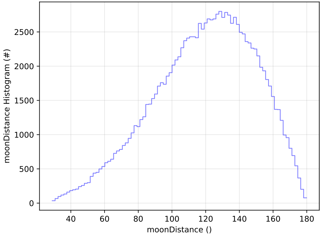
ddf_acor_sf30_lsf40_lsr20_v3.4_10yrs WFD u band: moonDistance Histogram
