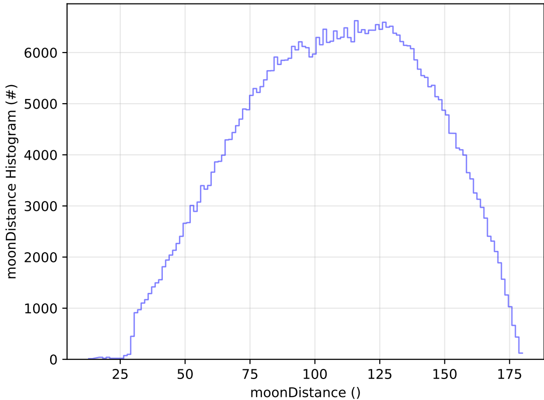
ddf_acor_sf30_lsf40_lsr20_v3.4_10yrs WFD r band: moonDistance Histogram
