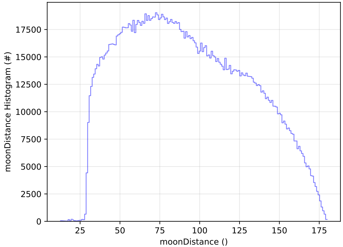
ddf_acor_sf30_lsf40_lsr20_v3.4_10yrs WFD all bands: moonDistance Histogram
