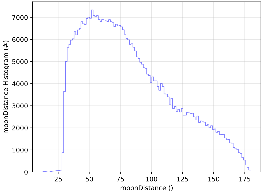
ddf_acor_sf30_lsf40_lsr20_v3.4_10yrs All sky z band: moonDistance Histogram
