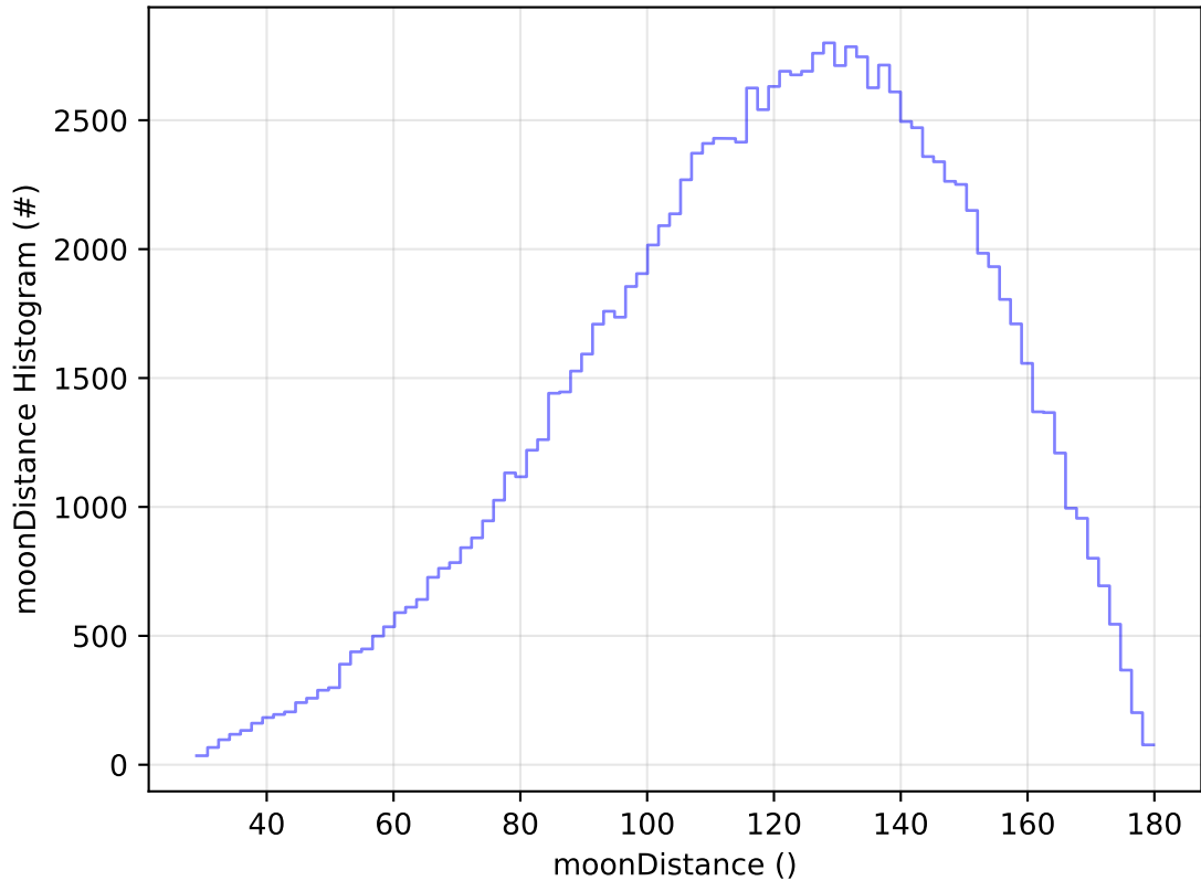
ddf_acor_sf30_lsf40_lsr20_v3.4_10yrs All sky u band: moonDistance Histogram
