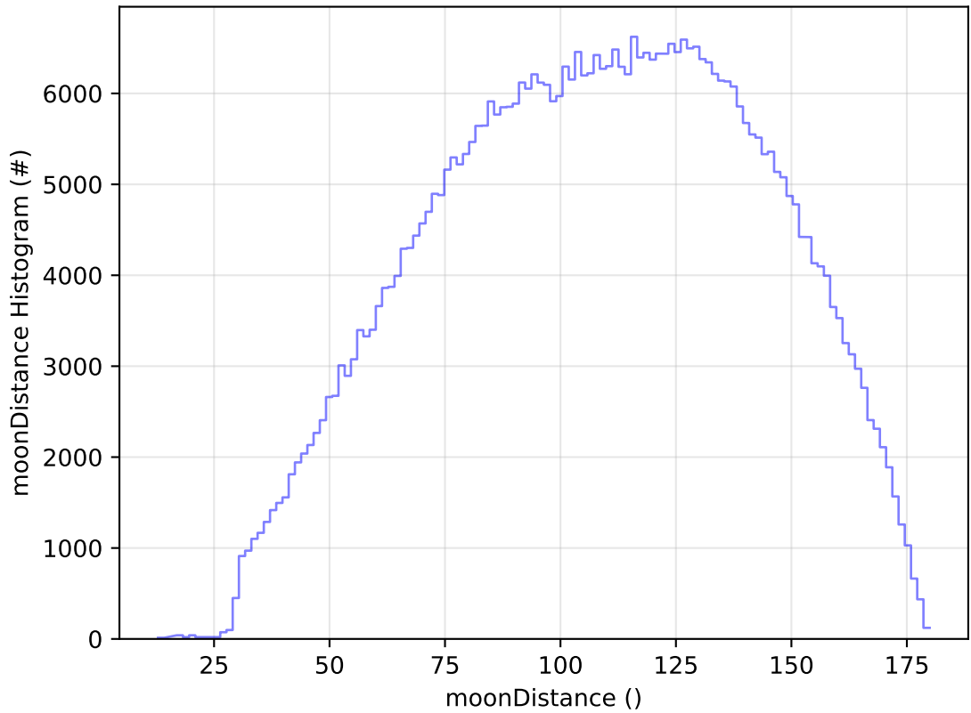
ddf_acor_sf30_Isf40_Isr20_v3.4_10yrs All sky r band: moonDistance Histogram
