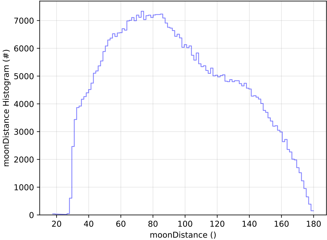
ddf_acor_sf30_lsf40_lsr20_v3.4_10yrs All sky i band: moonDistance Histogram
