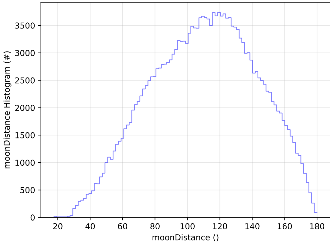
ddf_acor_sf30_lsf40_lsr20_v3.4_10yrs All sky g band: moonDistance Histogram
