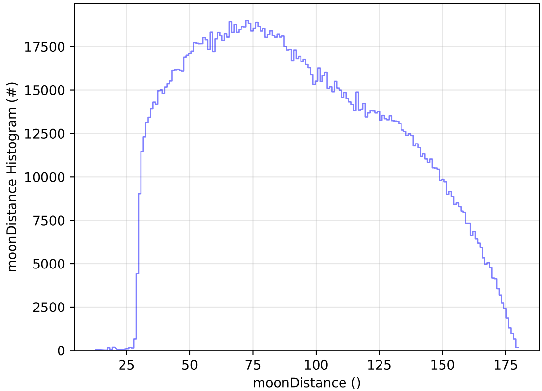
ddf_acor_sf30_lsf40_lsr20_v3.4_10yrs All sky all bands: moonDistance Histogram
