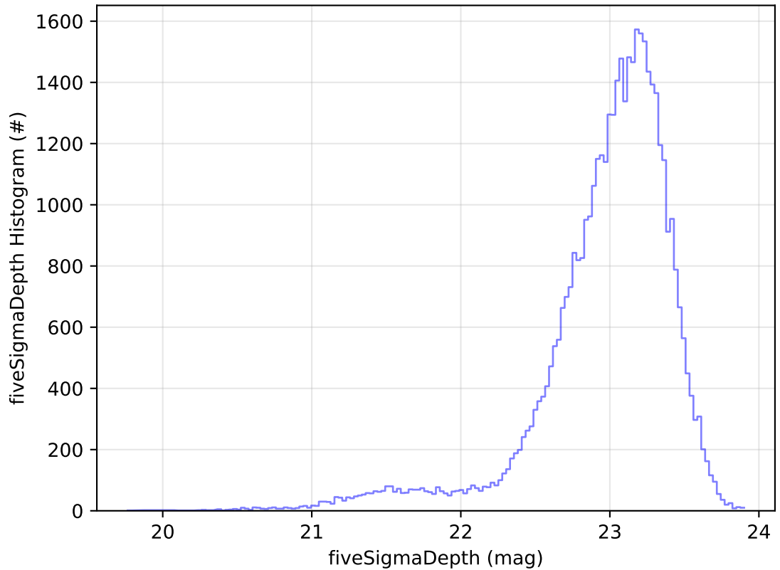
ddf_acor_sf30_lsf40_lsr20_v3.4_10yrs Yr 1 z band: fiveSigmaDepth Histogram
