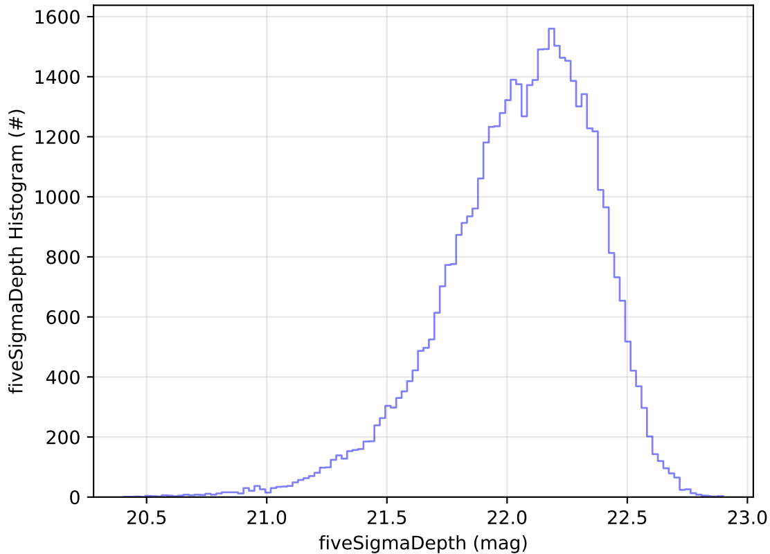
ddf_acor_sf30_lsf40_lsr20_v3.4_10yrs Yr 1 y band: fiveSigmaDepth Histogram
