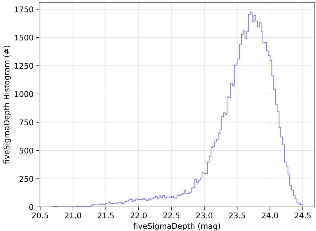
ddf_acor_sf30_lsf40_lsr20_v3.4_10yrs Yr 1 i band: fiveSigmaDepth Histogram
