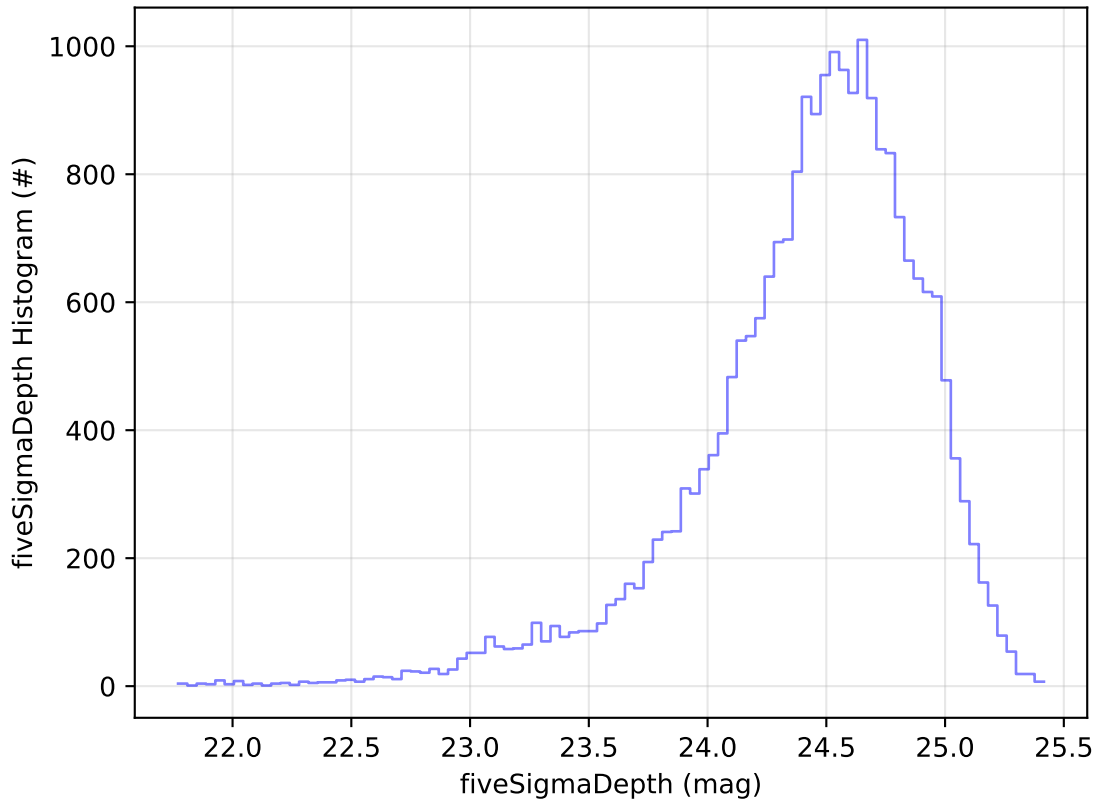
ddf_acor_sf30_lsf40_lsr20_v3.4_10yrs Yr 1 g band: fiveSigmaDepth Histogram
