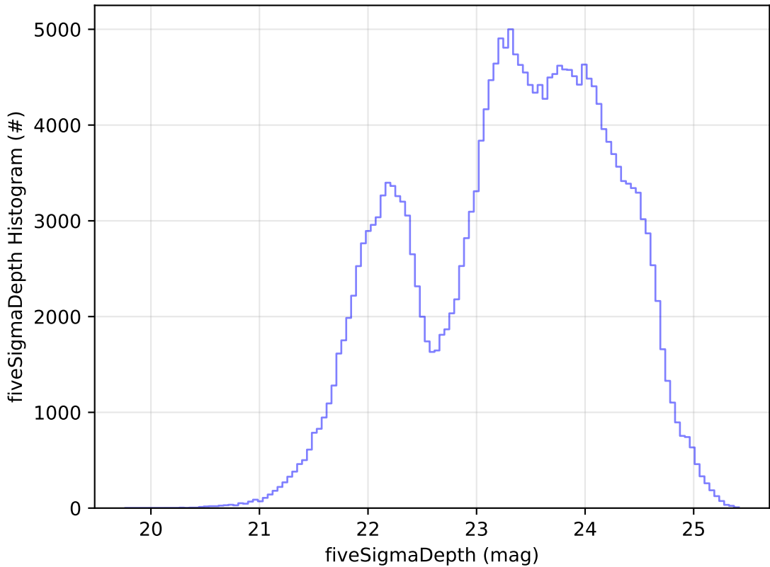
ddf_acor_sf30_Isf40_Isr20_v3.4_10yrs Yr 1 all bands: fiveSigmaDepth Histogram
