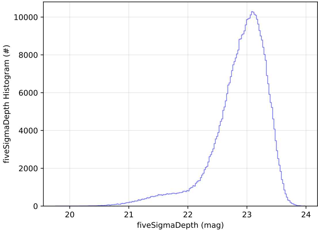
ddf_acor_sf30_lsf40_lsr20_v3.4_10yrs WFD z band: fiveSigmaDepth Histogram
