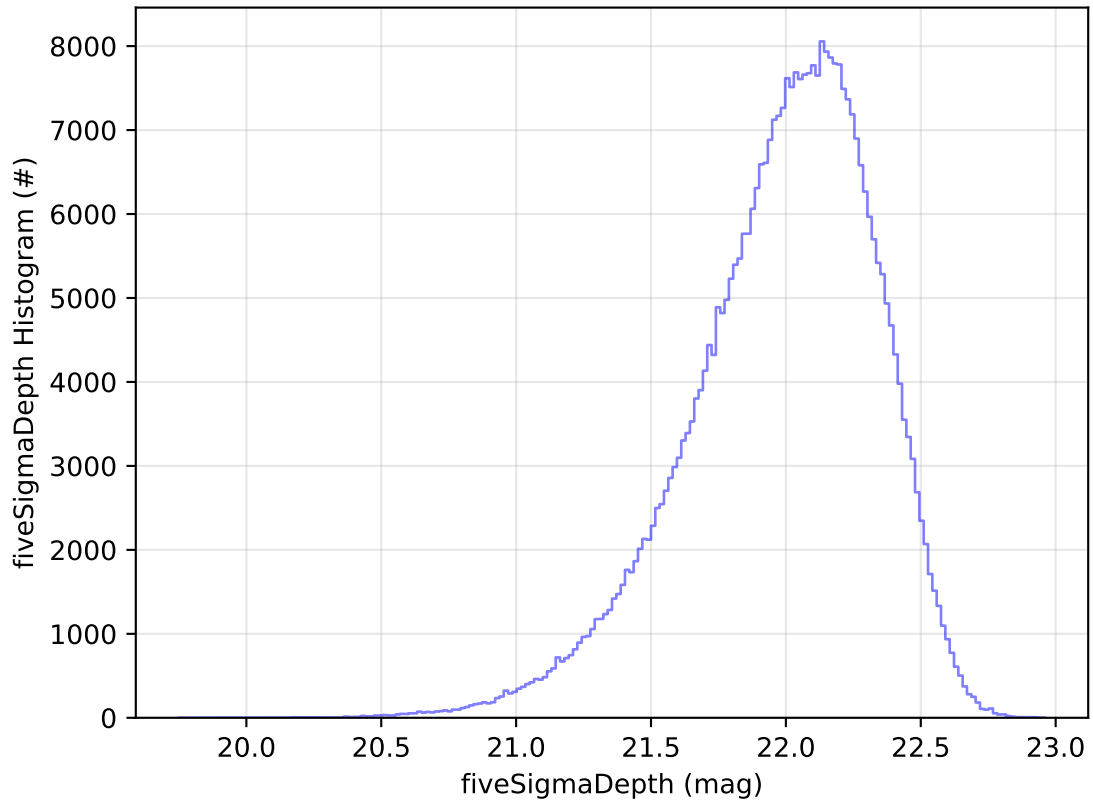
ddf_acor_sf30_lsf40_lsr20_v3.4_10yrs WFD y band: fiveSigmaDepth Histogram
