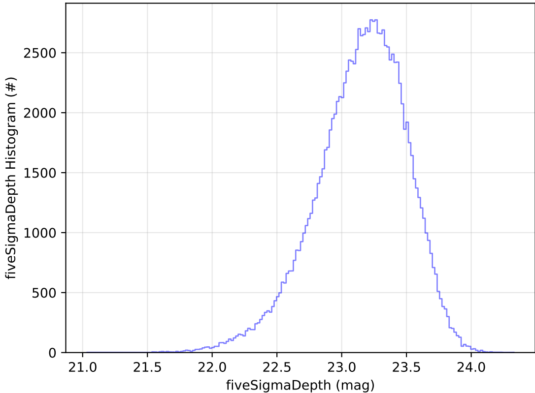
ddf_acor_sf30_lsf40_lsr20_v3.4_10yrs WFD u band: fiveSigmaDepth Histogram
