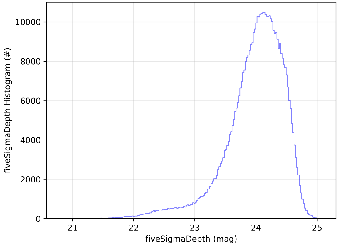
ddf_acor_sf30_lsf40_lsr20_v3.4_10yrs WFD r band: fiveSigmaDepth Histogram
