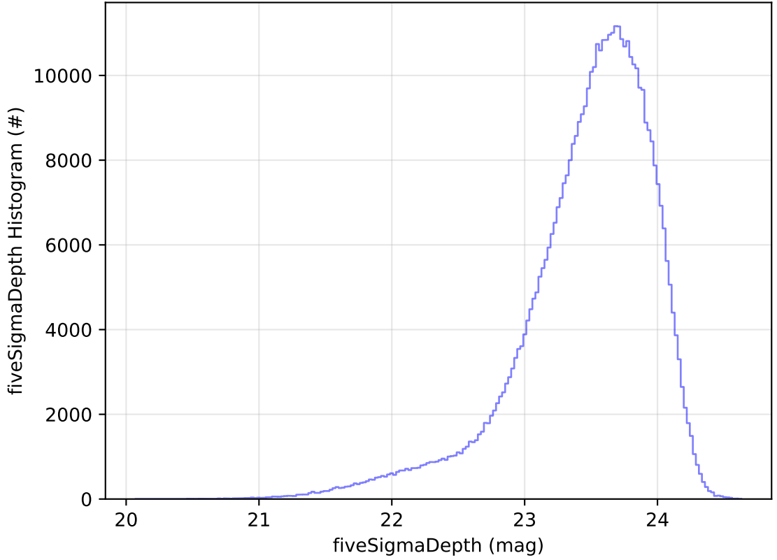
ddf_acor_sf30_lsf40_lsr20_v3.4_10yrs WFD i band: fiveSigmaDepth Histogram
