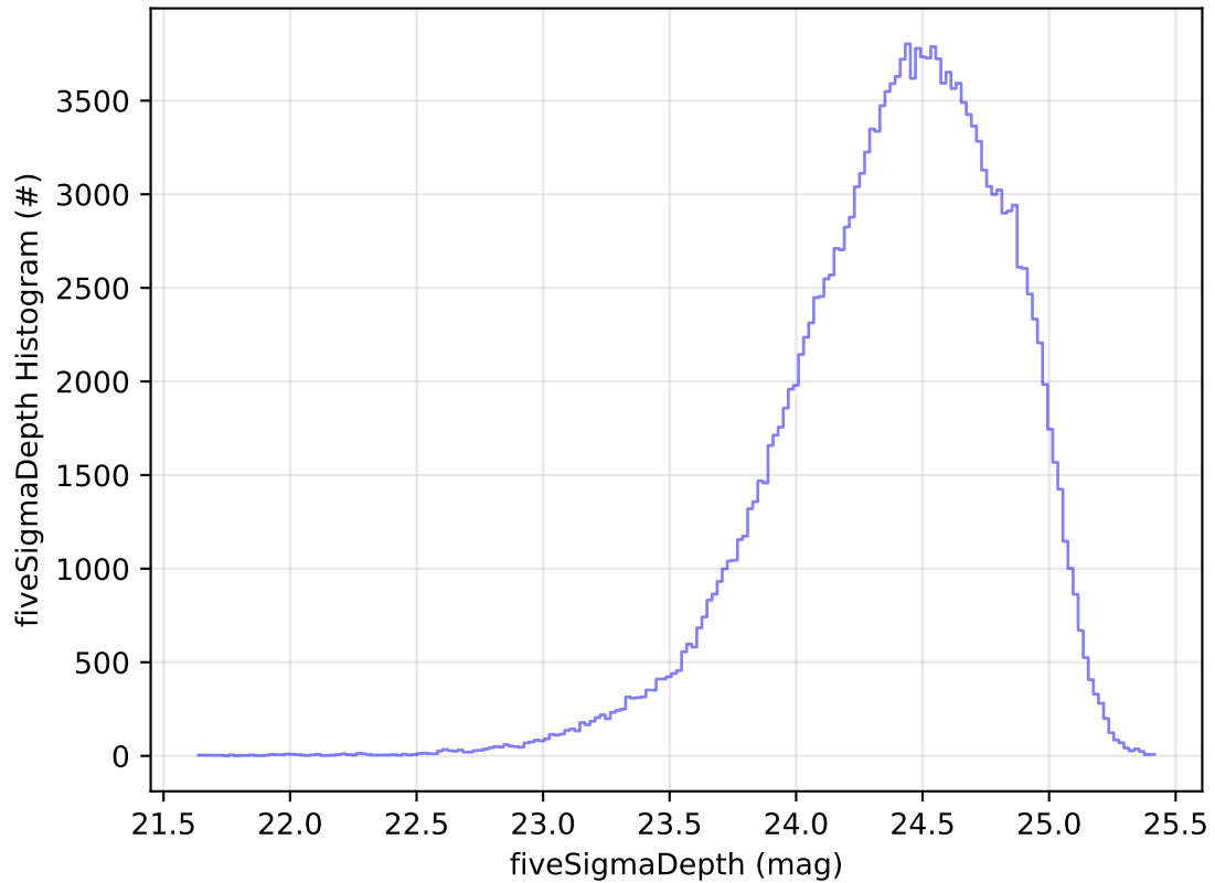
ddf_acor_sf30_lsf40_lsr20_v3.4_10yrs WFD g band: fiveSigmaDepth Histogram
