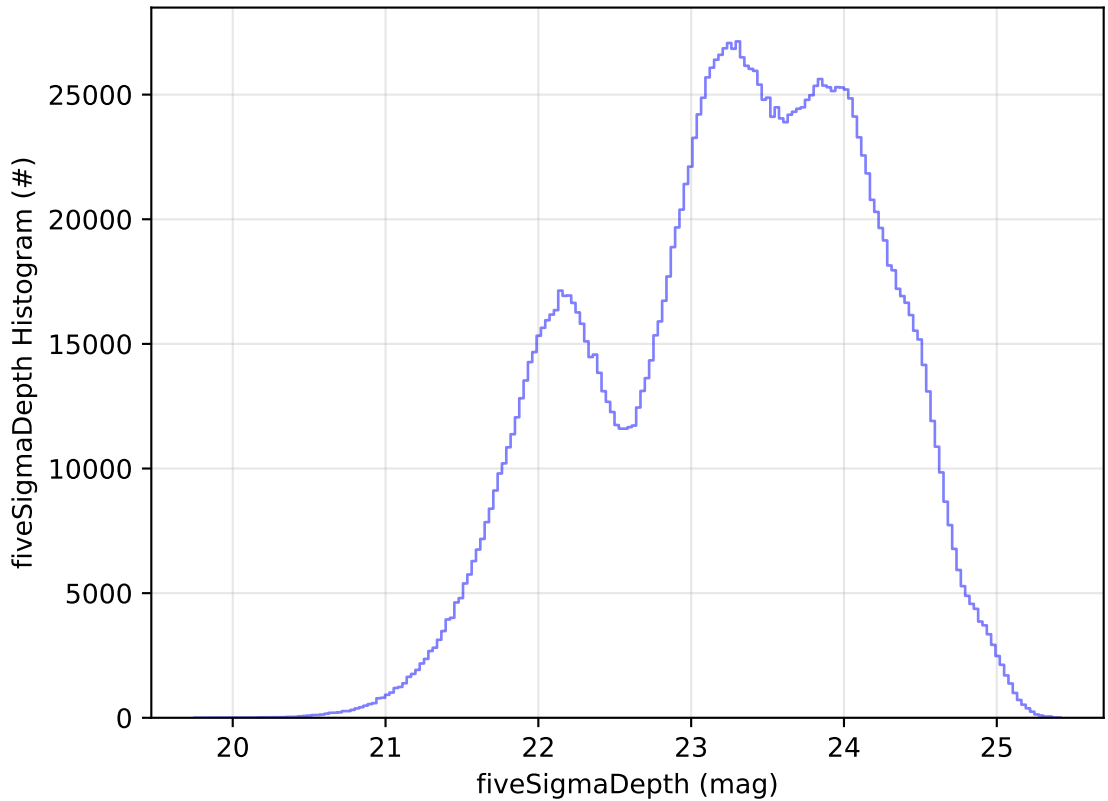
ddf_acor_sf30_lsf40_lsr20_v3.4_10yrs WFD all bands: fiveSigmaDepth Histogram
