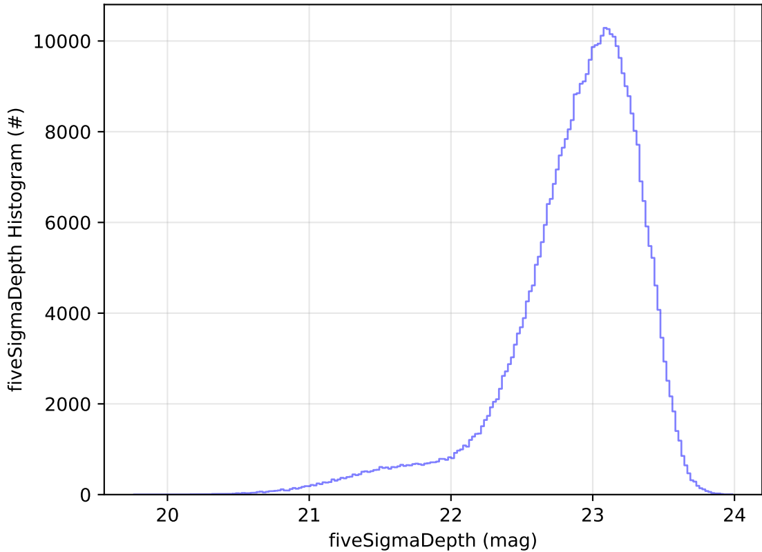
ddf_acor_sf30_lsf40_lsr20_v3.4_10yrs All sky z band: fiveSigmaDepth Histogram
