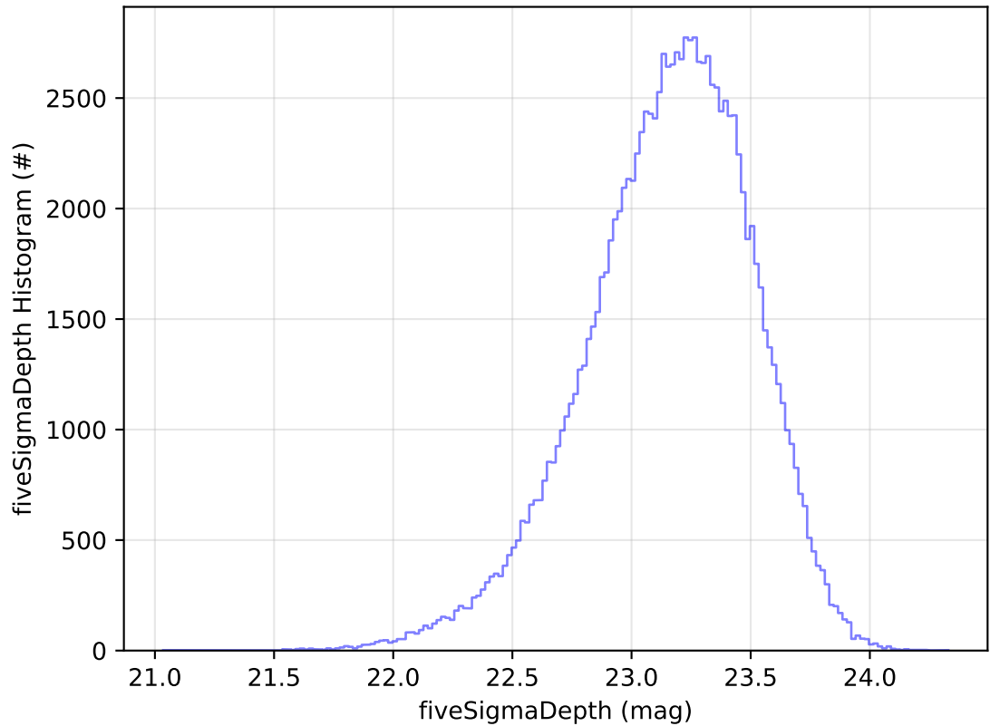
ddf_acor_sf30_lsf40_lsr20_v3.4_10yrs All sky u band: fiveSigmaDepth Histogram
