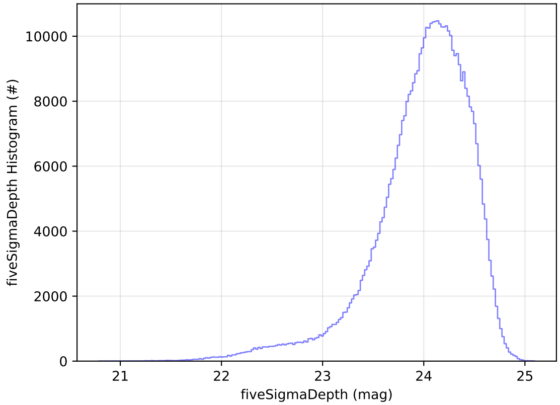
ddf_acor_sf30_lsf40_lsr20_v3.4_10yrs All sky r band: fiveSigmaDepth Histogram
