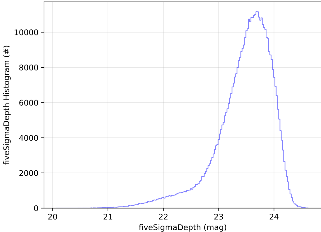
ddf_acor_sf30_lsf40_lsr20_v3.4_10yrs All sky i band: fiveSigmaDepth Histogram
