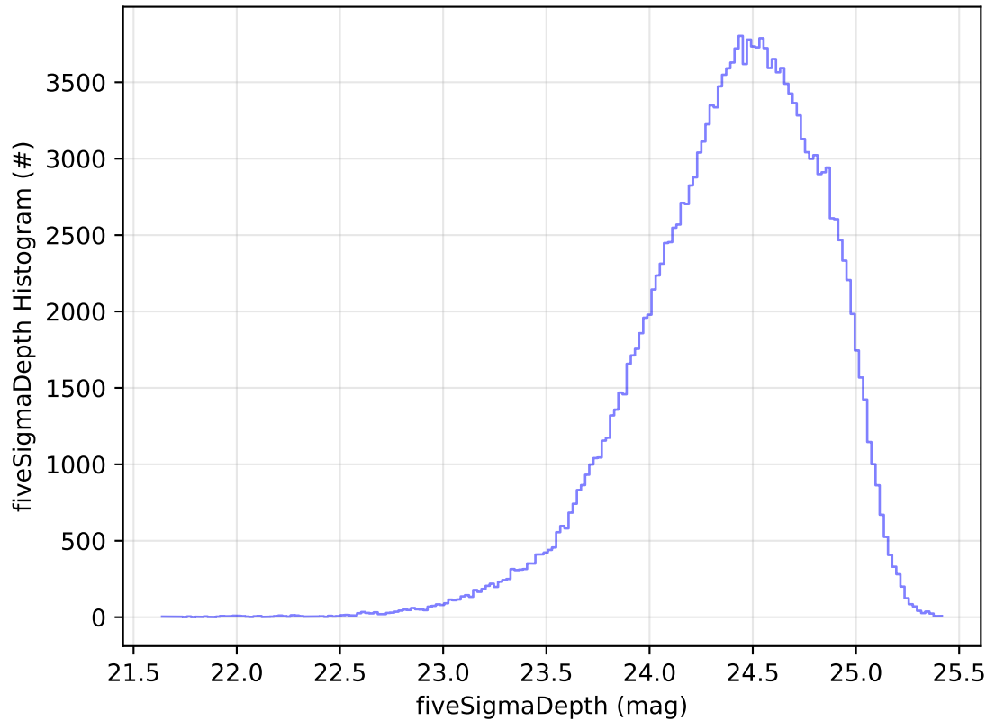
ddf_acor_sf30_lsf40_lsr20_v3.4_10yrs All sky g band: fiveSigmaDepth Histogram
