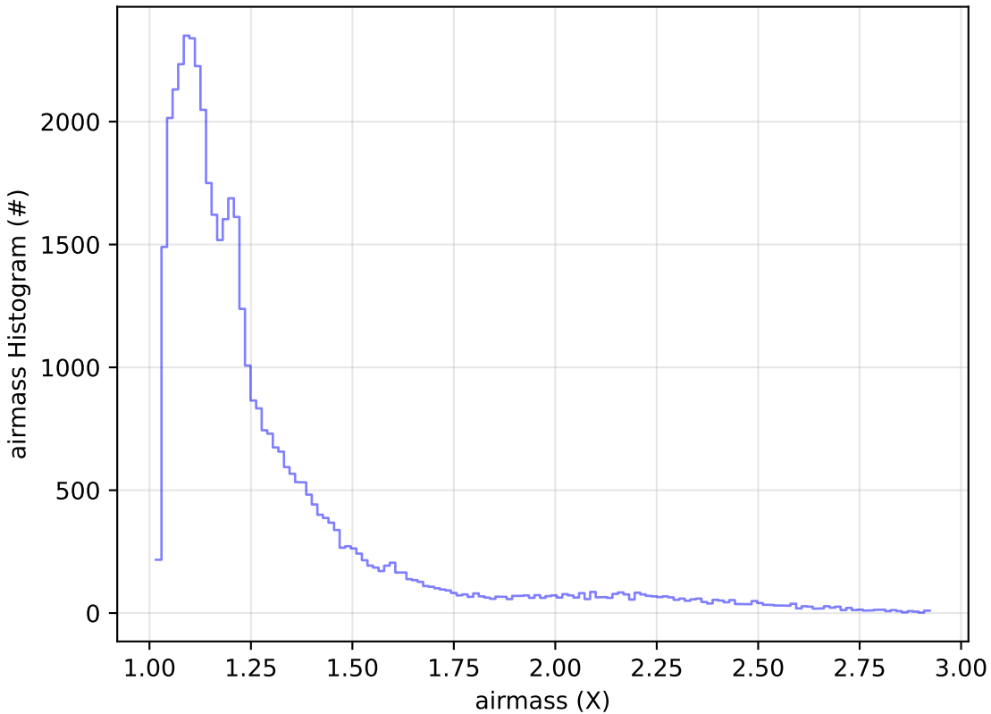
ddf_acor_sf30_lsf40_lsr20_v3.4_10yrs Yr 1 z band: airmass Histogram
