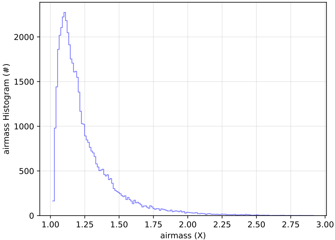
ddf_acor_sf30_lsf40_lsr20_v3.4_10yrs Yr 1 y band: airmass Histogram
