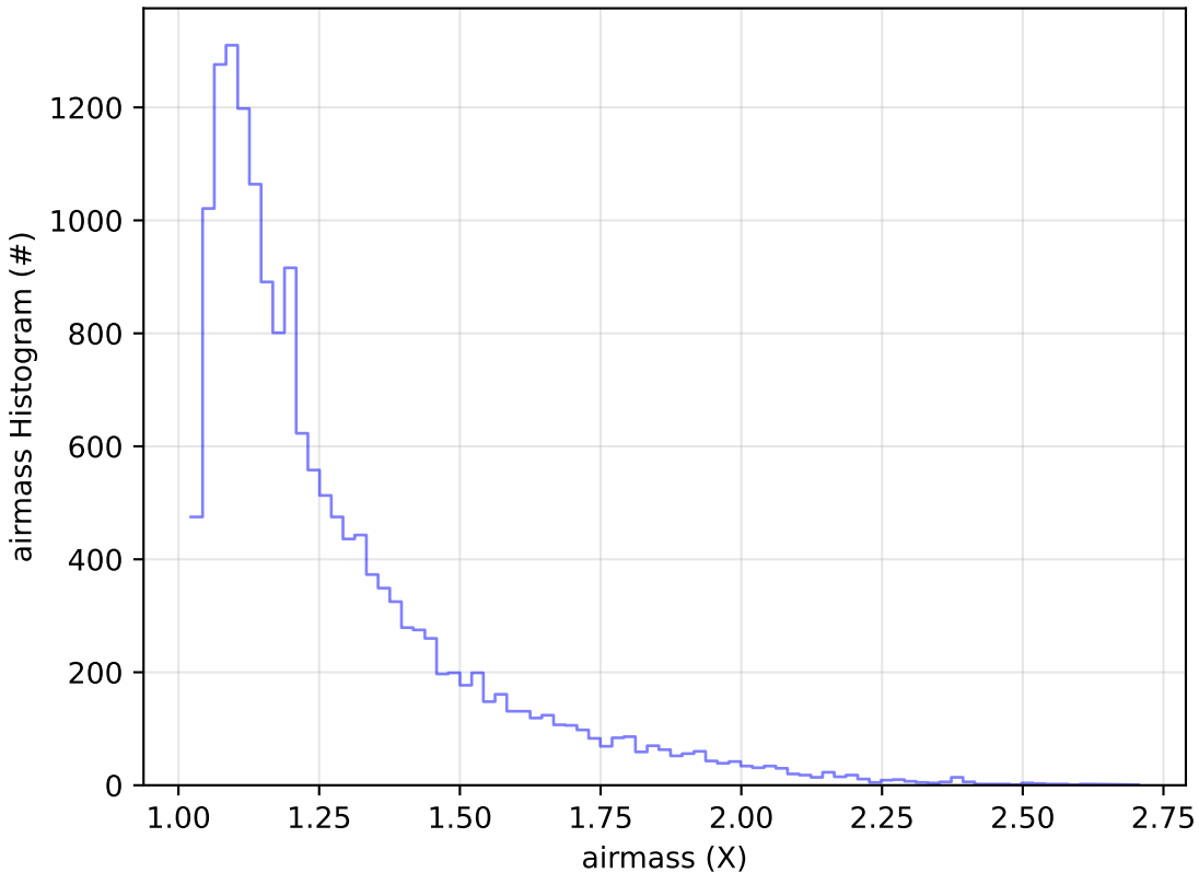
ddf_acor_sf30_lsf40_lsr20_v3.4_10yrs Yr 1 u band: airmass Histogram
