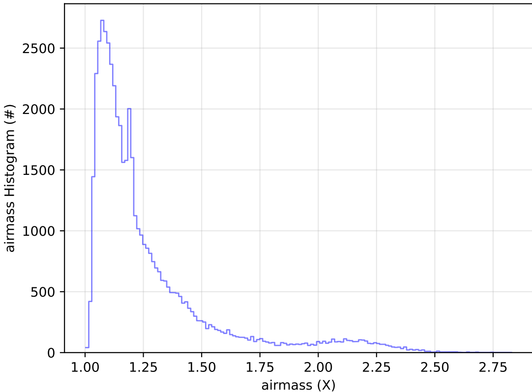
ddf_acor_sf30_Isf40_Isr20_v3.4_10yrs Yr 1 r band: airmass Histogram
