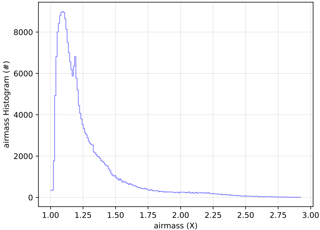
ddf_acor_sf30_lsf40_lsr20_v3.4_10yrs Yr 1 all bands: airmass Histogram
