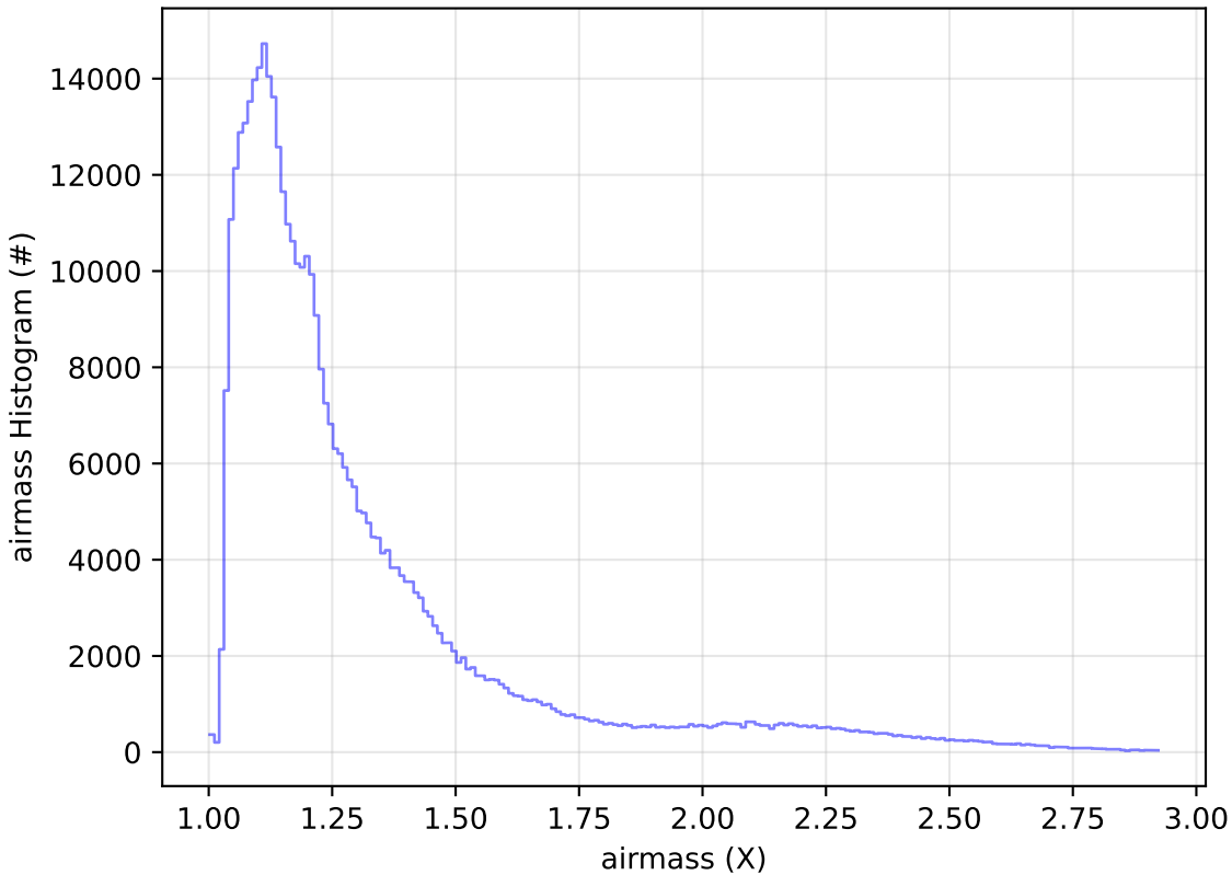
ddf_acor_sf30_lsf40_lsr20_v3.4_10yrs WFD z band: airmass Histogram
