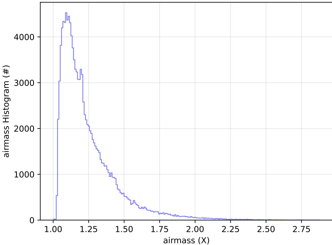
ddf_acor_sf30_lsf40_lsr20_v3.4_10yrs WFD u band: airmass Histogram
