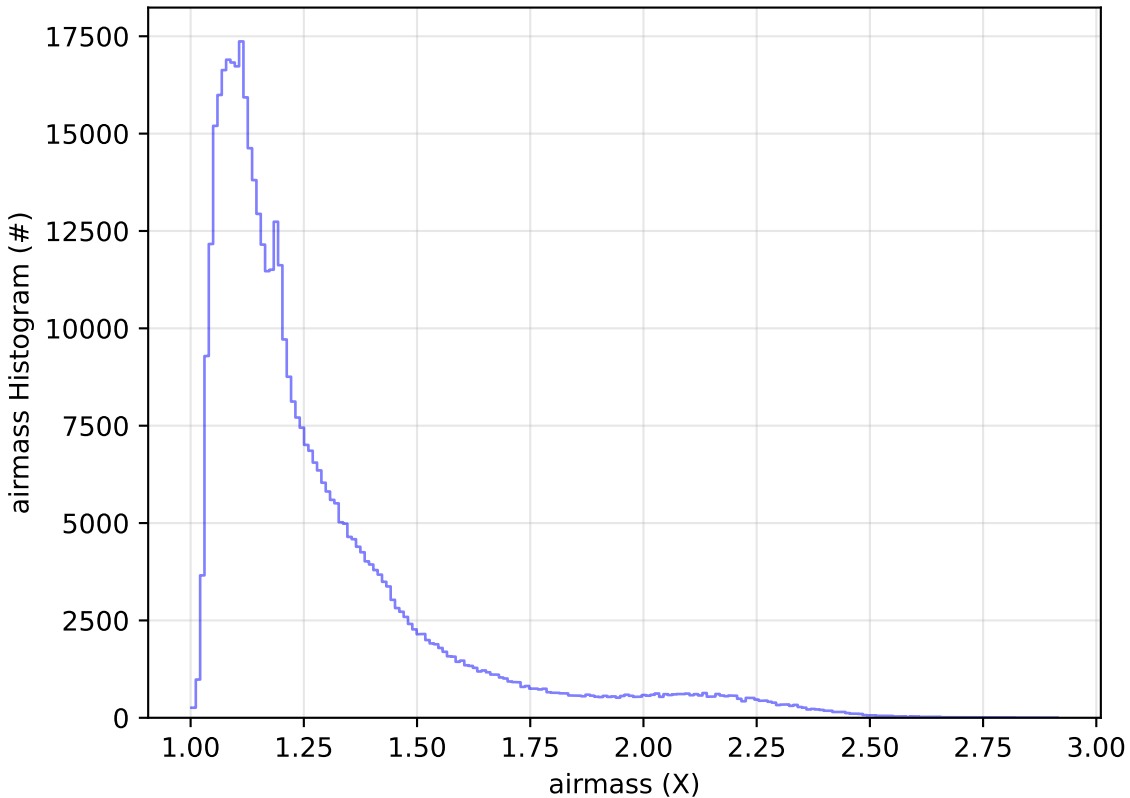
ddf_acor_sf30_Isf40_Isr20_v3.4_10yrs WFD r band: airmass Histogram
