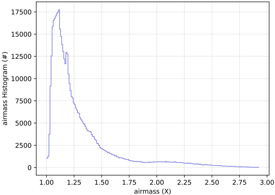
ddf_acor_sf30_lsf40_lsr20_v3.4_10yrs WFD i band: airmass Histogram
