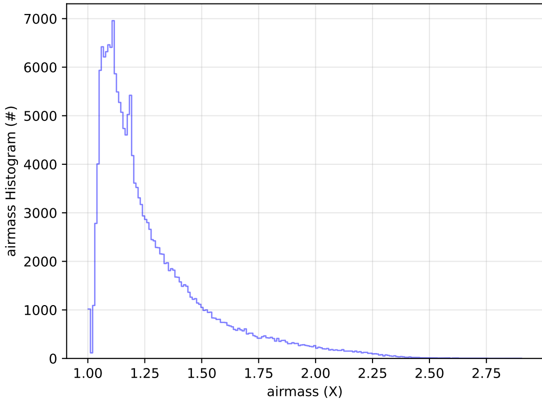
ddf_acor_sf30_lsf40_lsr20_v3.4_10yrs WFD g band: airmass Histogram
