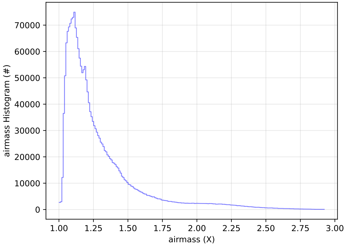
ddf_acor_sf30_lsf40_lsr20_v3.4_10yrs WFD all bands: airmass Histogram
