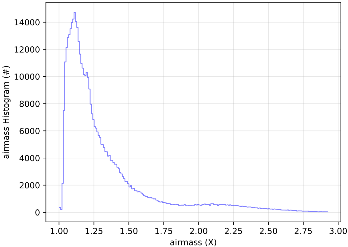
ddf_acor_sf30_lsf40_lsr20_v3.4_10yrs All sky z band: airmass Histogram
