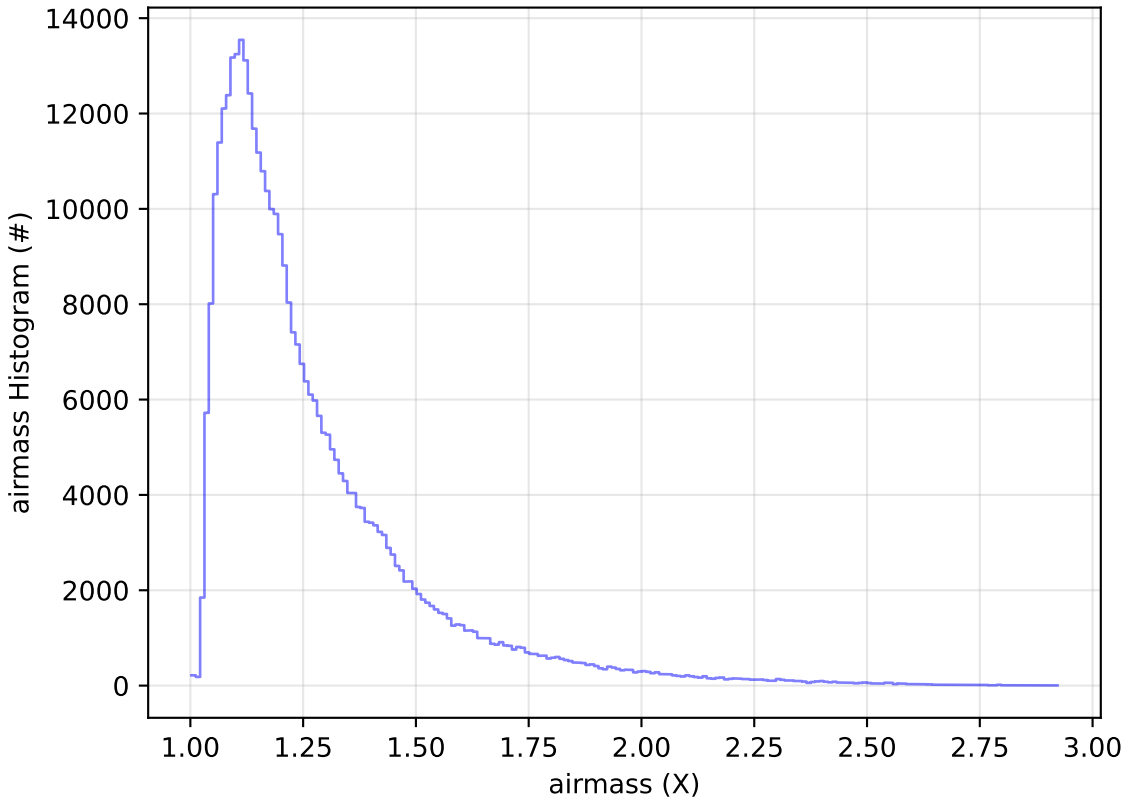
ddf_acor_sf30_lsf40_lsr20_v3.4_10yrs All sky y band: airmass Histogram
