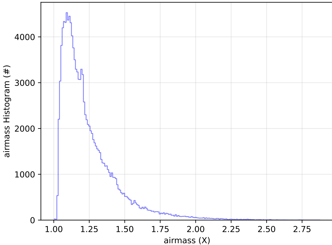
ddf_acor_sf30_lsf40_lsr20_v3.4_10yrs All sky u band: airmass Histogram
