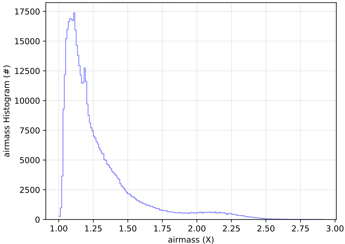
ddf_acor_sf30_lsf40_lsr20_v3.4_10yrs All sky r band: airmass Histogram
