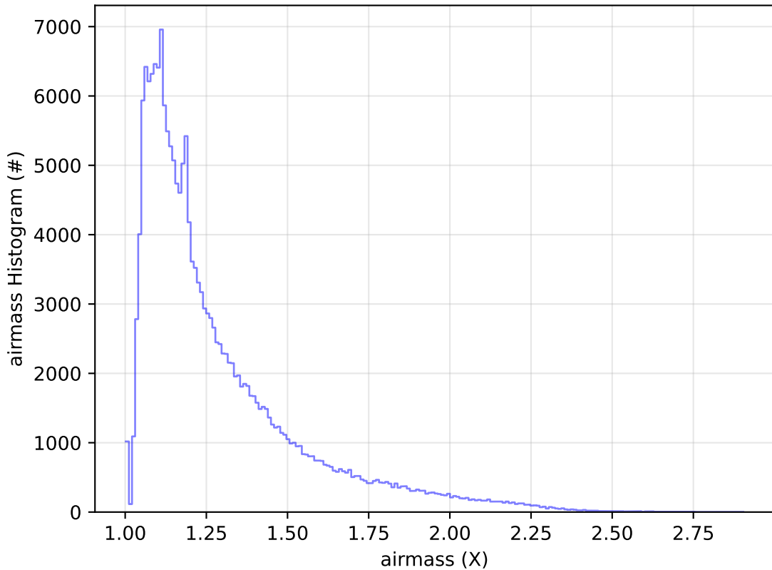
ddf_acor_sf30_lsf40_lsr20_v3.4_10yrs All sky g band: airmass Histogram
