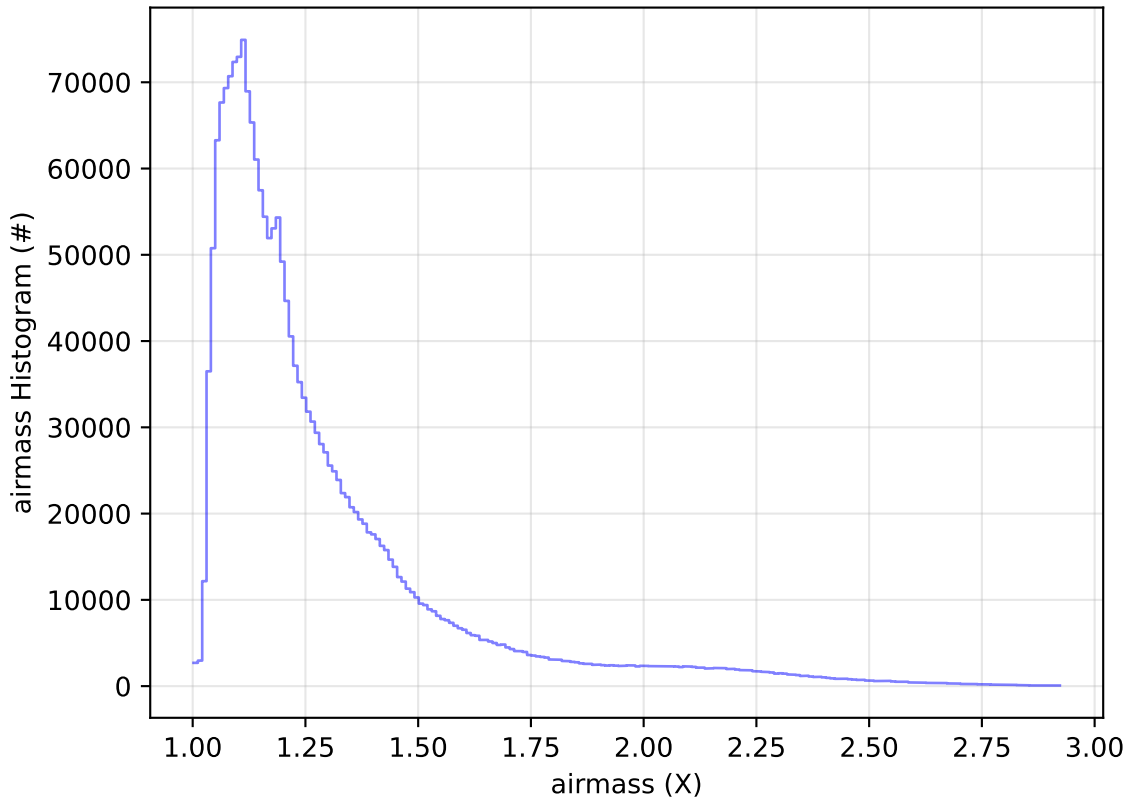
ddf_acor_sf30_lsf40_lsr20_v3.4_10yrs All sky all bands: airmass Histogram
