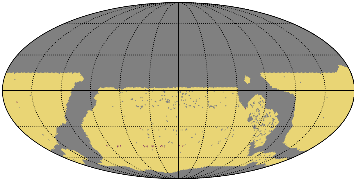
ddf_acor_sf30_lsf40_lsr20_v3.4_10yrs WFD: RapidRevisits
