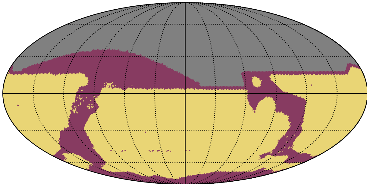
ddf_acor_sf30_lsf40_lsr20_v3.4_10yrs All sky: RapidRevisits
